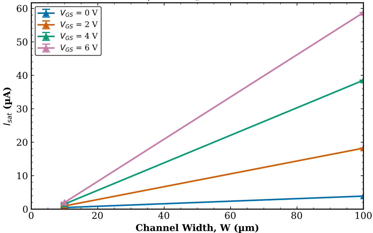
TFT3 Combined (Tr. 1 & 2) I_{sat} vs W | L = 8\text{ }\mu\text{m} (mean \pm std)
